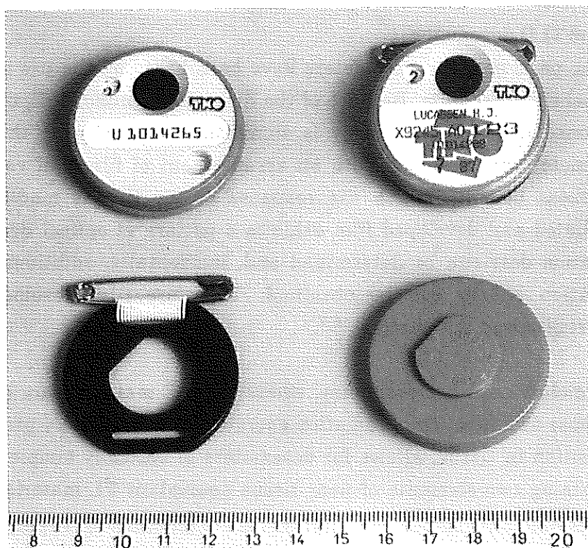
Fig. 3. The TNO TLD dosemeter, with and without the wearer's lable, showing the individual's name, number and issuing period
