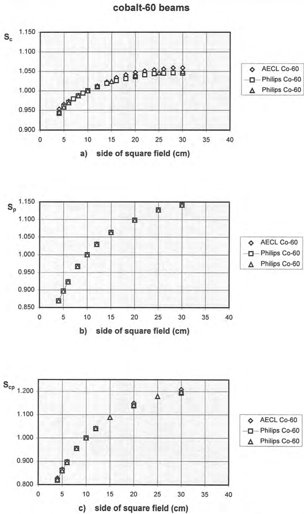
Figure 5.1 S_c , S_p and S_{cp} data as a function of the side of a square field of 60 Co beams (beams 1-3). Data are normalized at depth d_{ref} .
